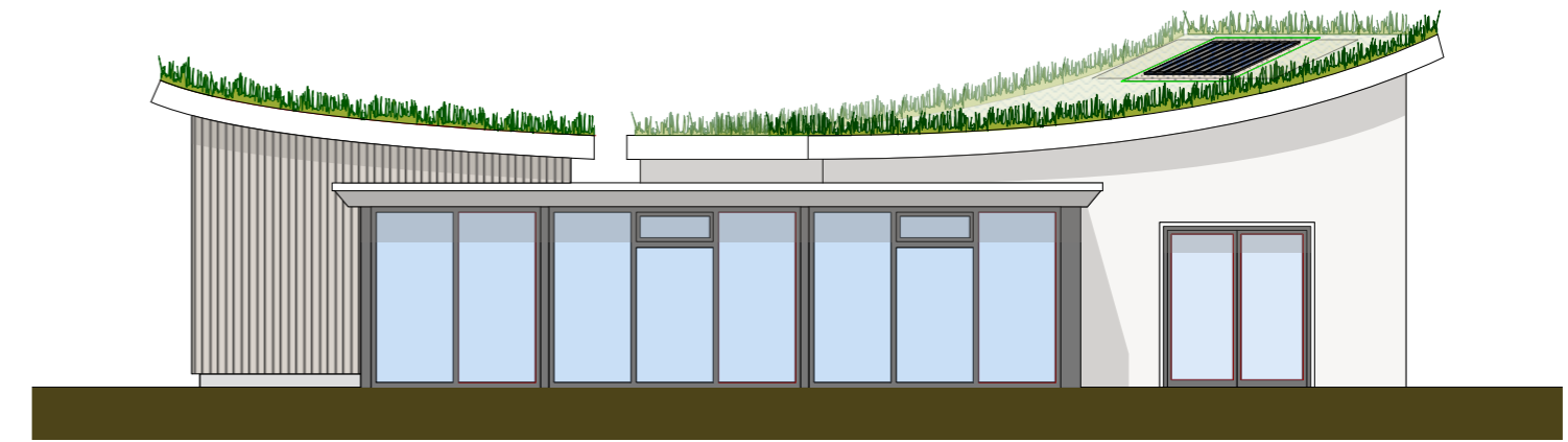
NORTH ELEVATION
